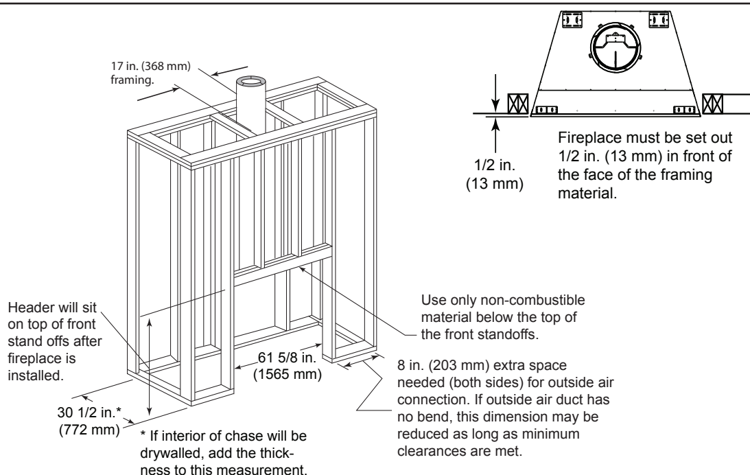
Figure 3.12 Framing the Fireplace
