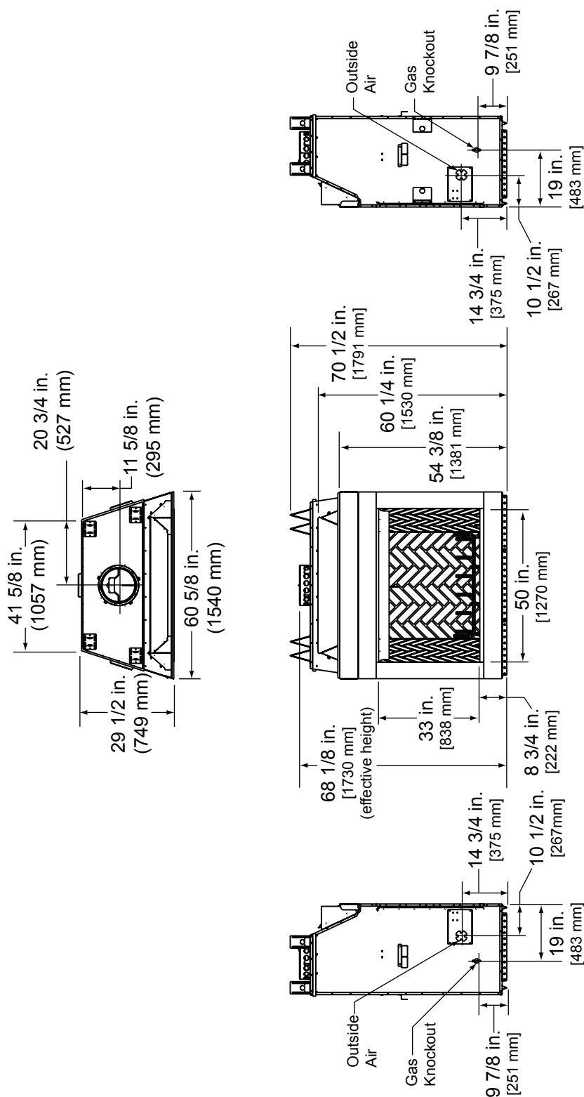
Figure 3.1 Fireplace Dimensions
